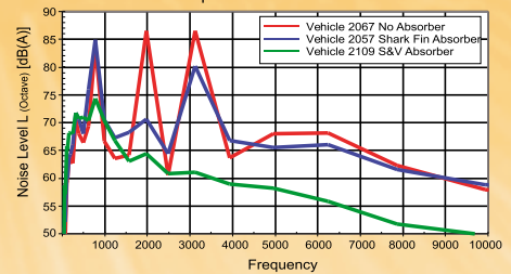
GVB Combino Tram pass by noise measurement Azarptlein/Amsterdam 03.09.04
